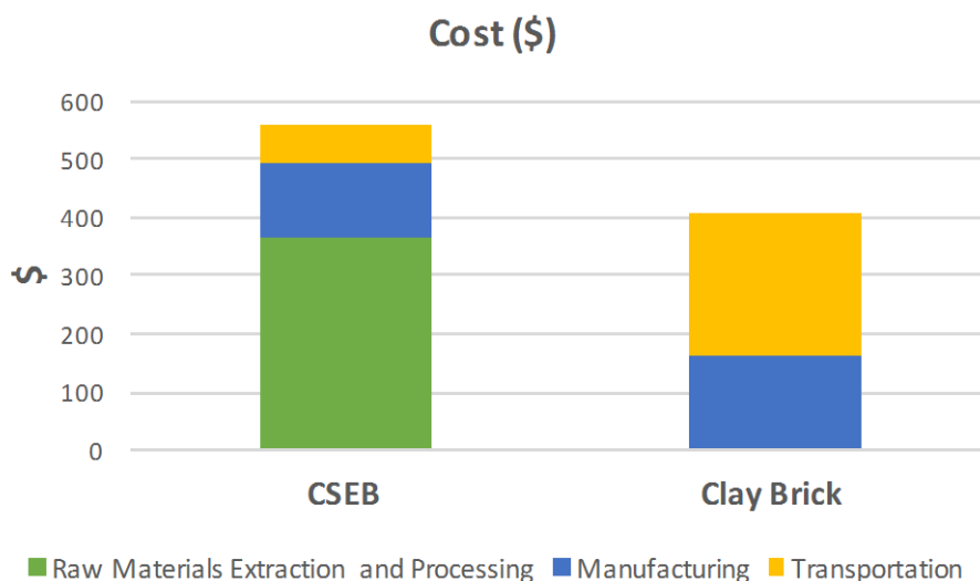
Figure 5-3: Results of LCA – Cost Comparison
