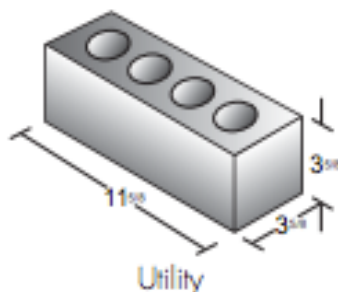
Figure 4-4: Typical Clay brick used in this study
