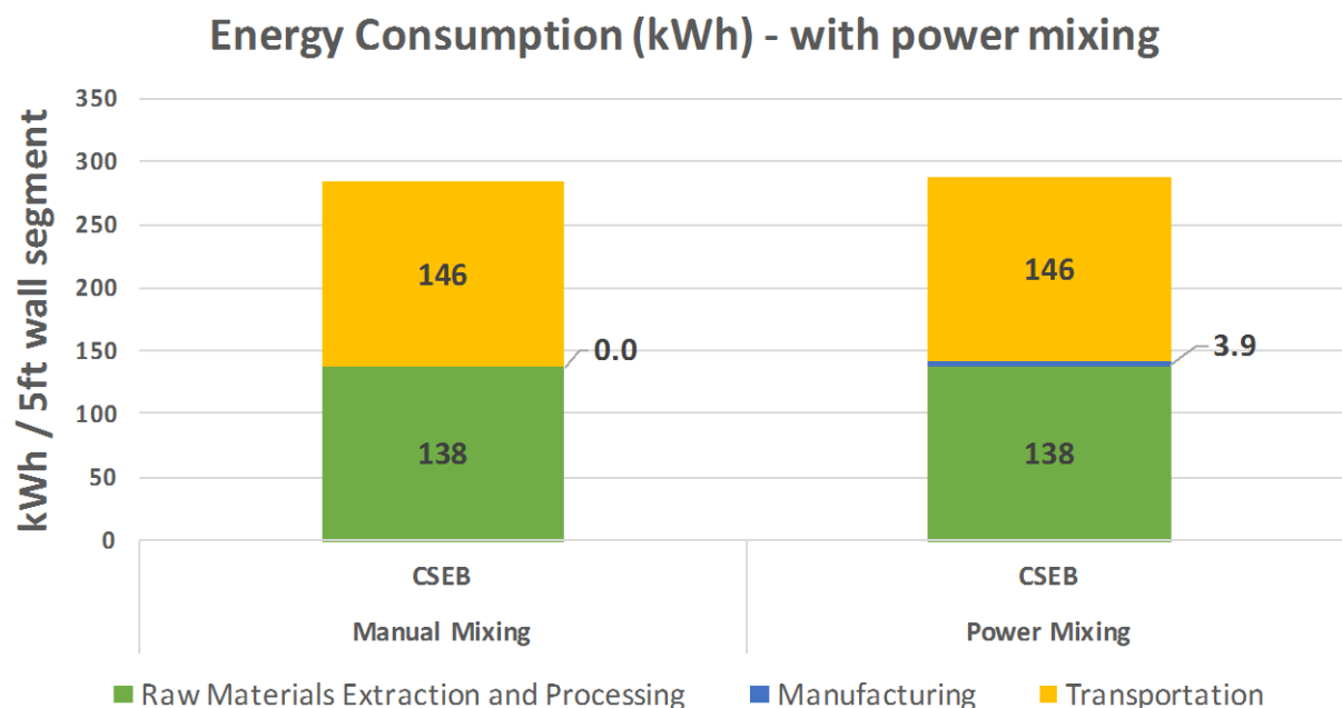
Figure 6-2: Sensitivity to use of power drill in CSEB mixing
