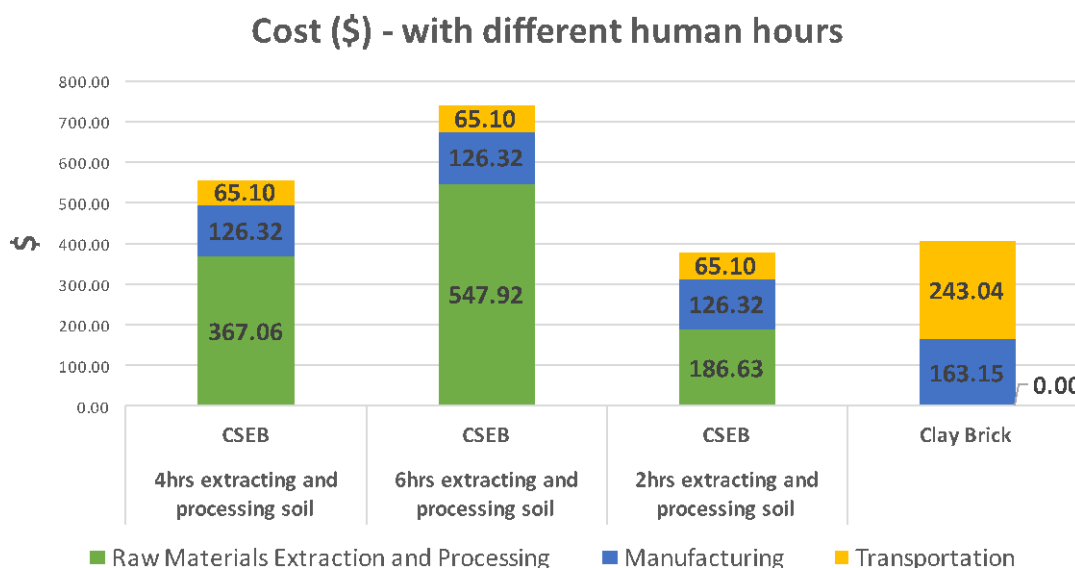
Figure 6-1: Sensitivity to varying labor efficiency in CSEB raw material extraction
