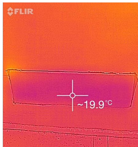
Figure 3-12: Infrared image of CSEB from inside protective chamber during heating
