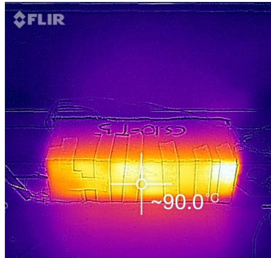
Figure 3-11: Infrared image of uncovered CSEB during heating
