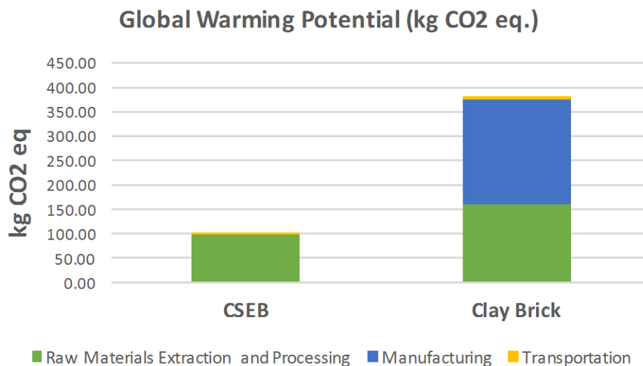
Figure 5-2: Results of LCA - Global Warming Potential (GWP) Comparison
