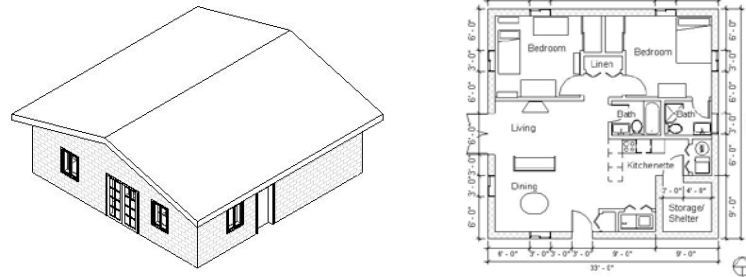
Figure 4-1: Single family dwelling in 3D (left) and plan view (right) (Erdogmus et al. 2015a)
