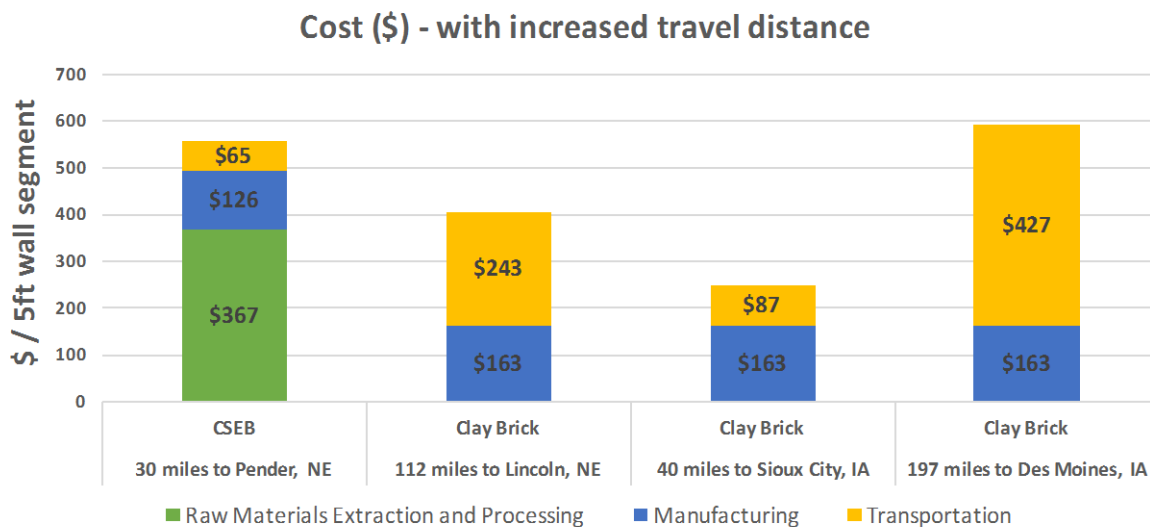
Figure 6-3: Sensitivity to increased travel distance of clay brick
