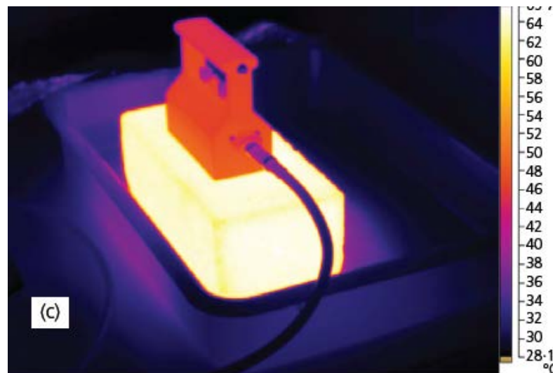
Figure 2-1: Transient Hot Wire Method used in Balaji et. al. 2016
