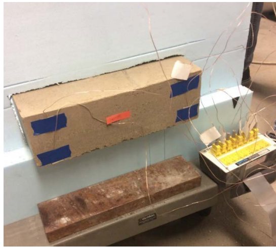
Figure 3-6: Thermocouples on exterior of CSEB
