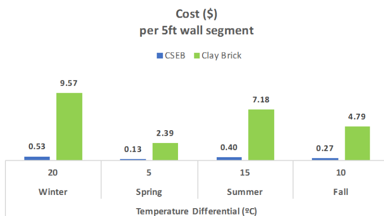
Figure 7-3: Thermal Conductivity: Cost ($) per 5ft wall segment
