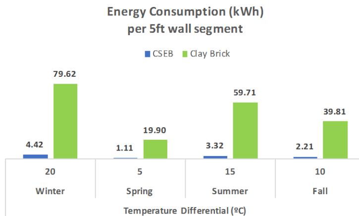
Figure 7-1: Thermal Conductivity: Energy Consumption (kWh) per 5ft wall segment
