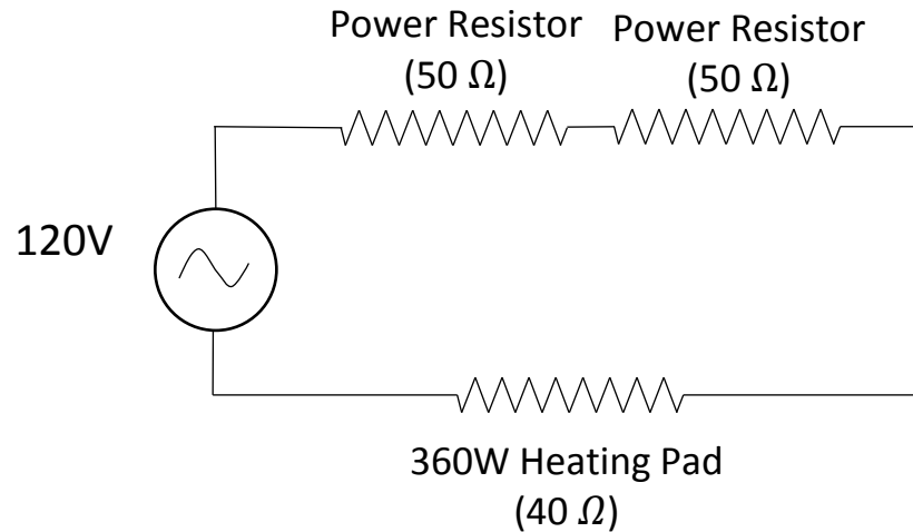
Figure 3-9: Schematic circuit diagram
