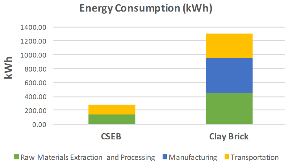
Figure 5-1: Results of LCA - Energy Consumption Comparison
